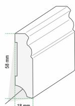
0040 Berliner skirting 58 mm Length 2,400 mm EAN 4250055116447
