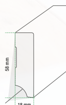
0038 Weimarer skirting 58 mm Length 2,400 mm EAN 4250055116324
