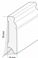
0041 Berliner skirting 78 mm Length 2,400 mm EAN 4250055116454
