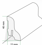
0026 Skirting white 40 mm Length 2,400 mm EAN 4250055101740
